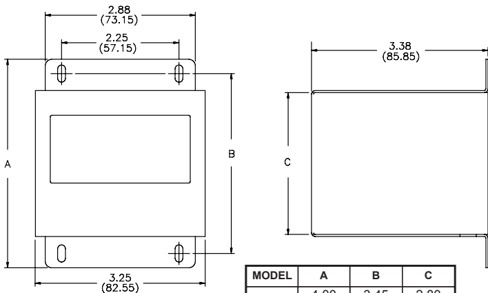
BMK7/BMK7A - CLOSED BASE MOUNT KIT (With or Without MLPS)
